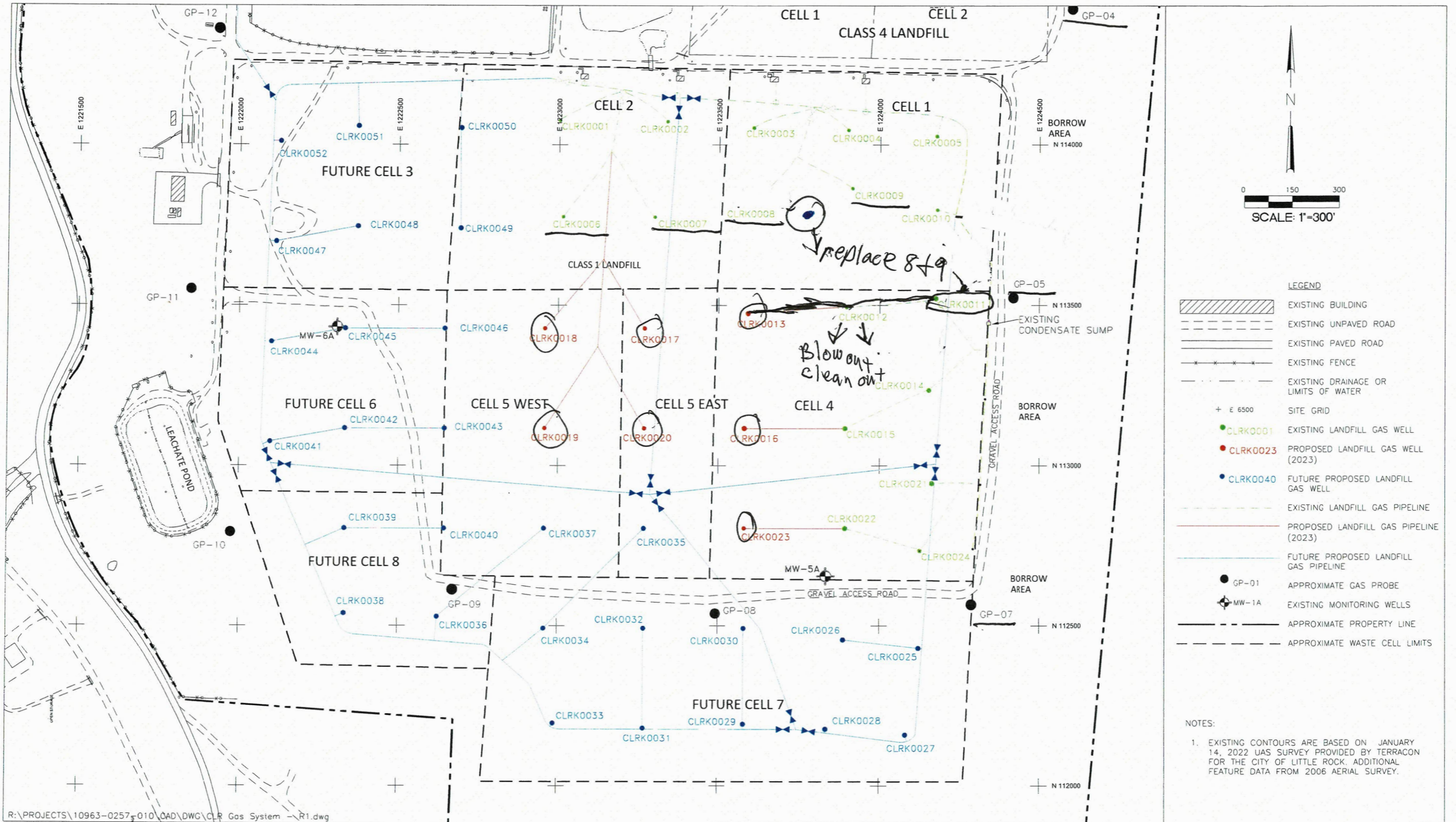
Figure 1. Existing and Proposed LFG Wells
